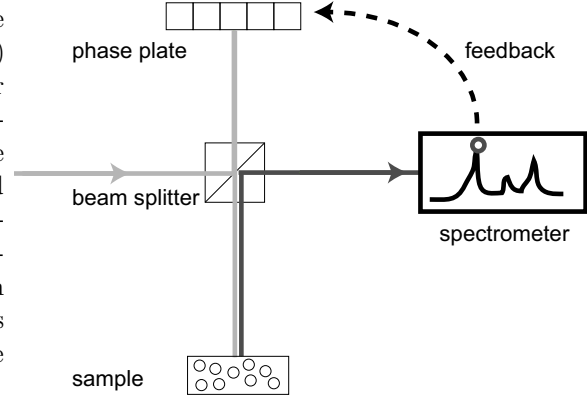
Figure 7.4: Sketch of experimental setup for wavefront shaping random lasers. The wave profile of the pump light (gray arrows) is modulated by a Spatial Light Modulator (SLM). The modulated phase front is projected onto the random laser sample. The emission light (dark gray arrows) is detected using a spectrometer. The intensity of a narrow spectral feature is used as a feedback signal for the amplitude and phase distribution on the SLM. An optimization algorithm is then employed to increase the signal of the selected narrow spectral feature.
