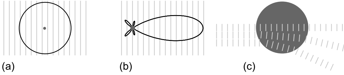
Figure 1.5: The size of a scatterer determines its scattering function. (a) For particles much smaller than the wavelength the scattering is governed by Rayleigh scattering. The scattering is isotropic in the plane perpendicular to the polarization. (b) Particles with a size on the order of the wavelength are in the Mie-regime. The scattering function is very dependent on angle. (c) When the size of the particle is much larger than the wavelength ray optics can be used to describe the scattering process.
