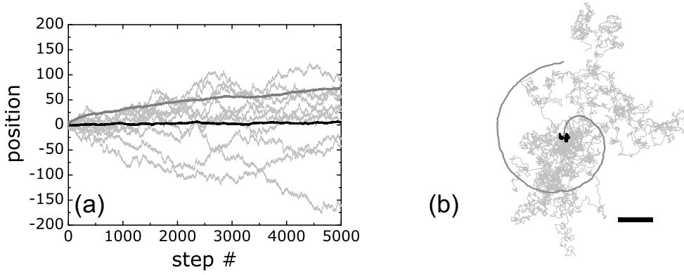
Figure 1.7: Random walks in (a) 1D and (b) 2D with unit step size. The light gray curves are examples of 10 random walks in 1D and 8 in 2D with 5000 and 500 steps respectively. The black curves are the ensemble averages over 100 samples. The dark gray curves indicate the root mean square of the displacement, which has been parameterized in the 2D case. The black bar equals 10 unit steps.
