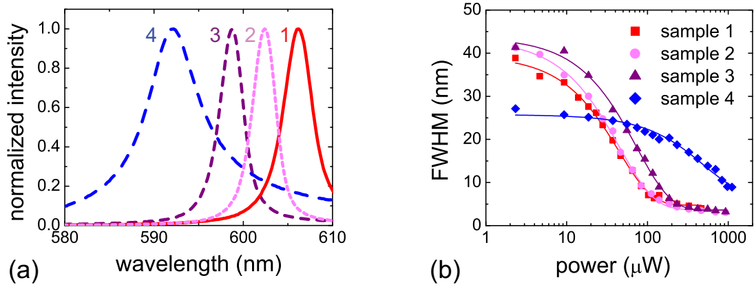
Figure 5.2: (a) emission spectrum above threshold for random laser samples 1-4. Pump powers: 465 \mu\text{W} for sample 1, 930 \mu\text{W} for sample 2 and 3, and 1114 \mu\text{W} for sample 4. (b) Width of the spectrum versus pump power for random laser samples 1-4.
