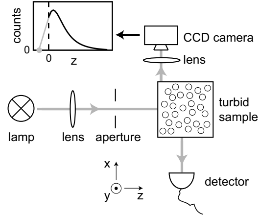
Figure 7.3: Turbidimeter based on the method of extrapolation. Light from an incoherent light source is incident on a turbid sample. A detector placed at 90 degrees with respect to the incident beam forms a conventional nephelometer. This part of the apparatus is used to measure the turbidity of weakly scattering samples. For multiple scattering media (samples with high turbidity), the turbidity is measured by imaging the side of the sample onto a CCD camera. Extrapolation of the diffuse intensity to zero intensity, as illustrated in the graph, returns the extrapolation length indicated by the gray dot. From the extrapolation length the transport mean free path is deduced which is a direct measure for the turbidity of the sample.
